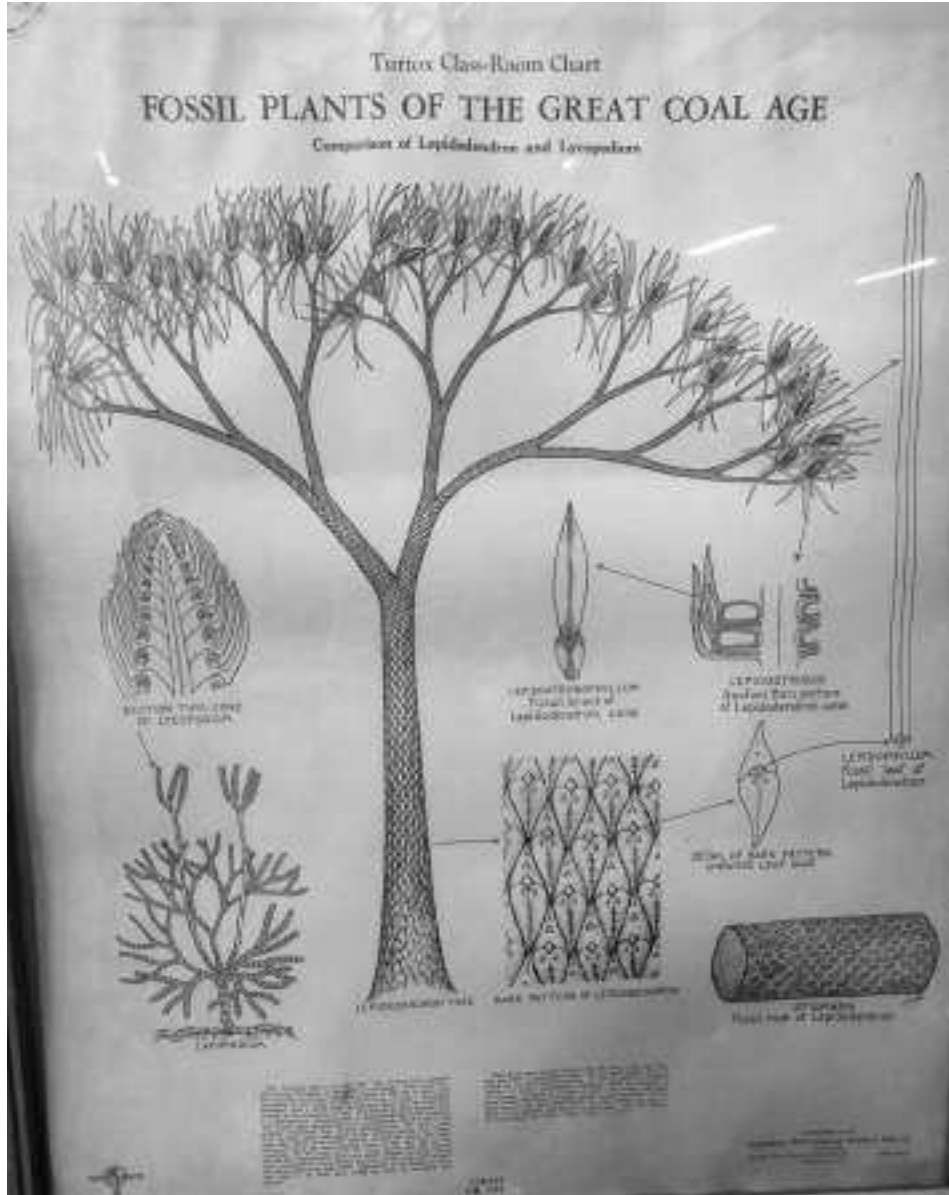
28/02/2024: Morphological and anatomical representation of fossil plant from the Great Coal Age.
